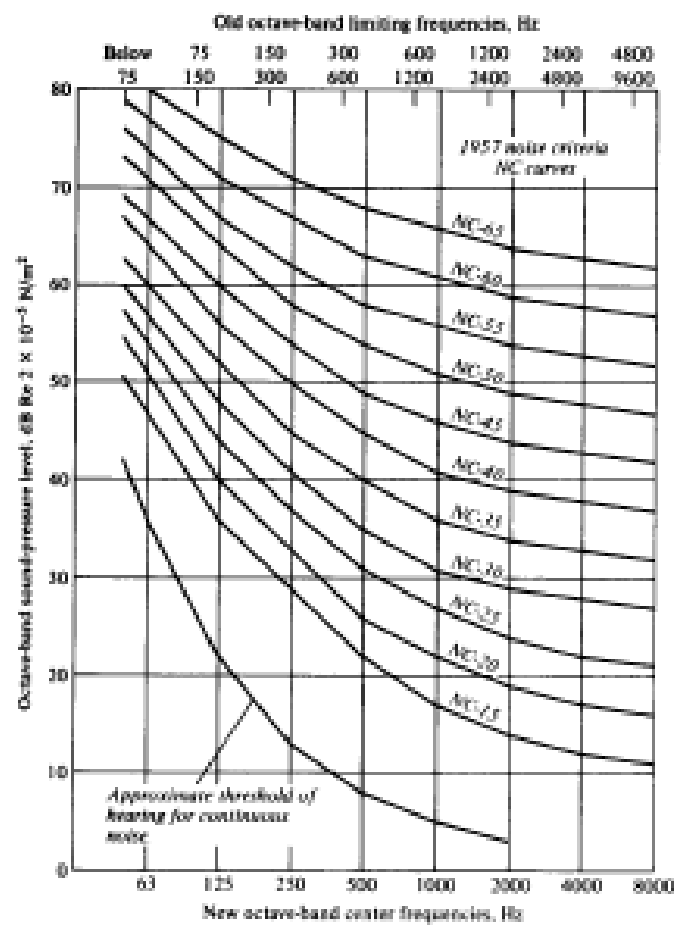
Figure 7.1 Indoor noise criteria (NC) curves (1957) [9].
