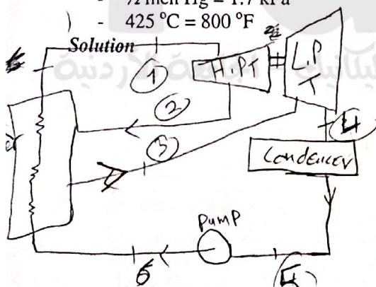
a) Cycle sketch
